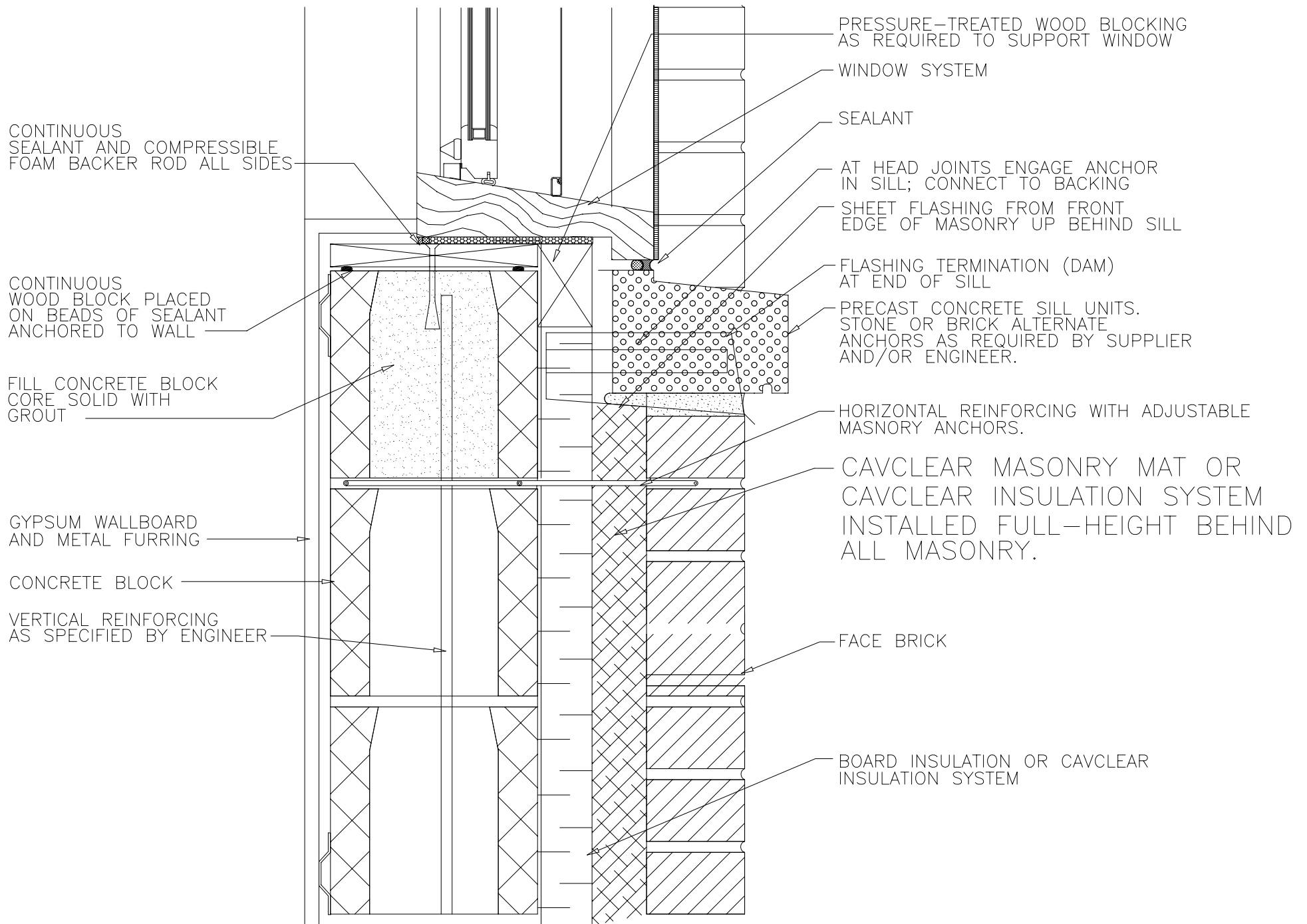
WINDOW SILL DETAIL (WOOD)
