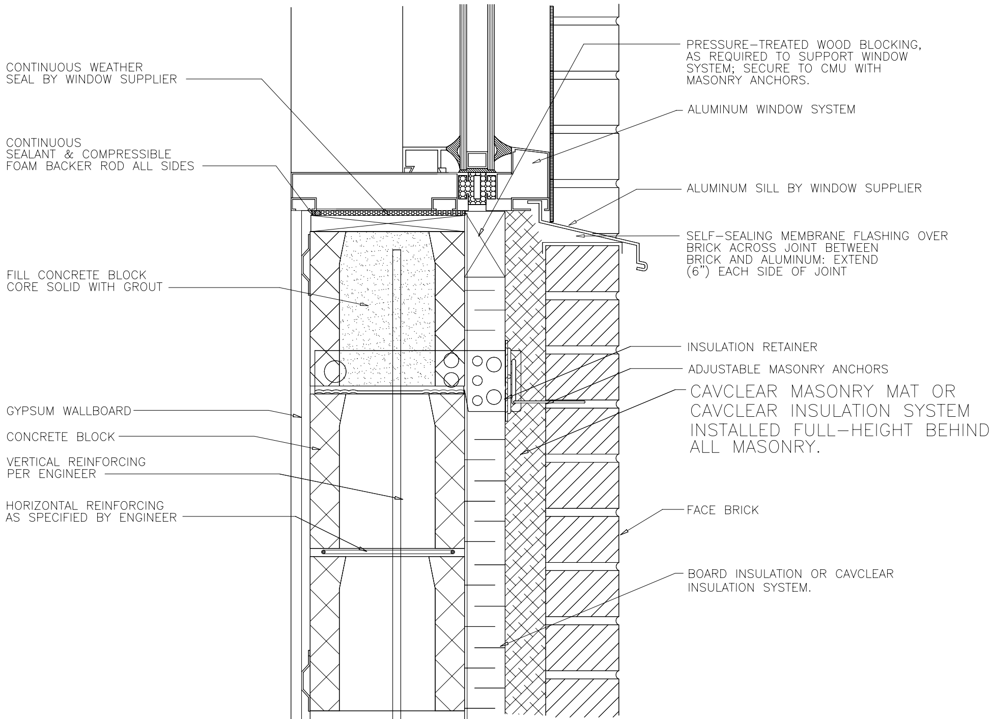
WINDOW SILL DETAIL (ALUMINUM)
