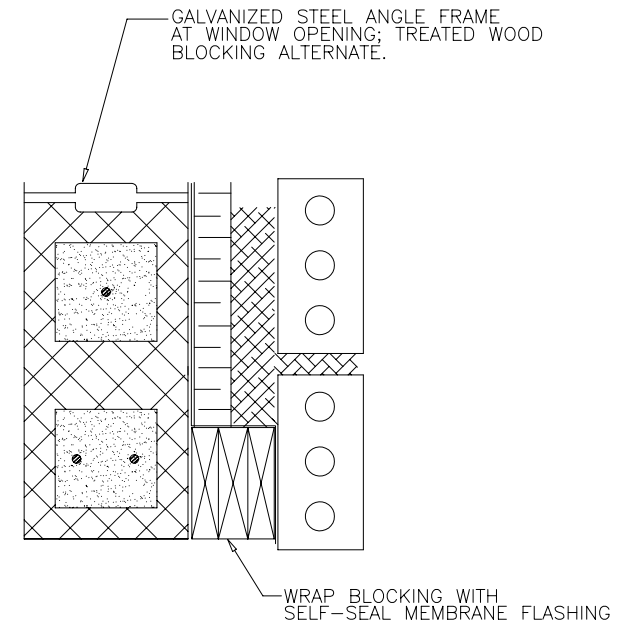
ALTERNATE WITH WOOD BLOCKING AT JAMB
