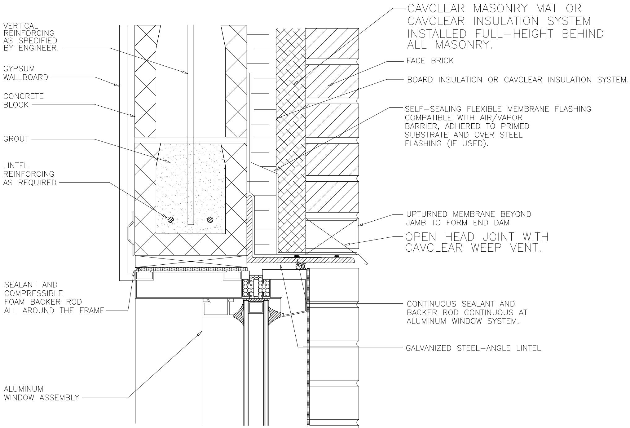
WINDOW HEAD DETAIL (ALUMINUM)
